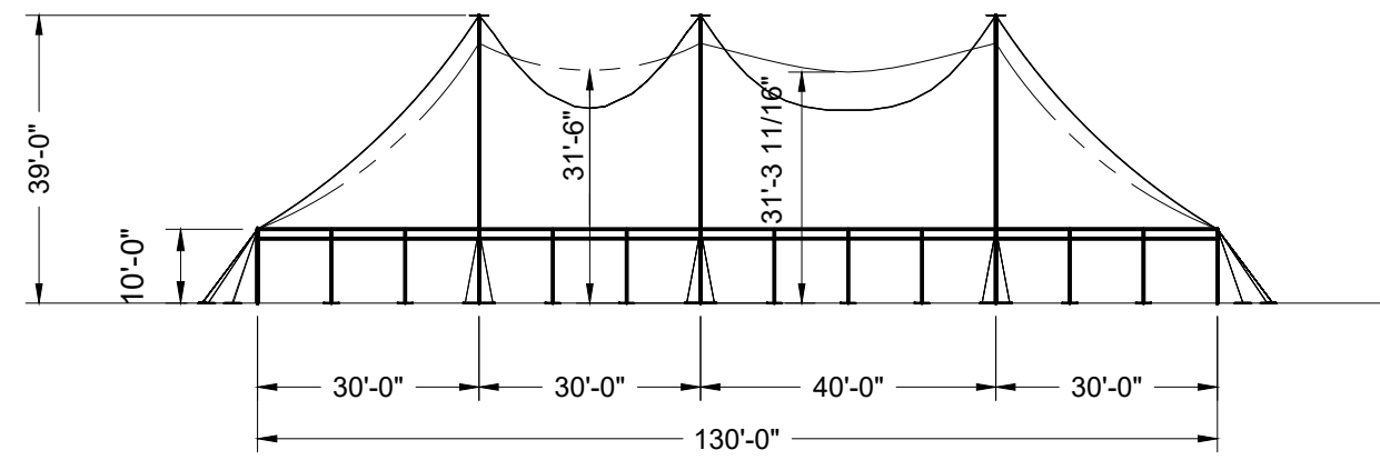
SIDE ELEVATION
