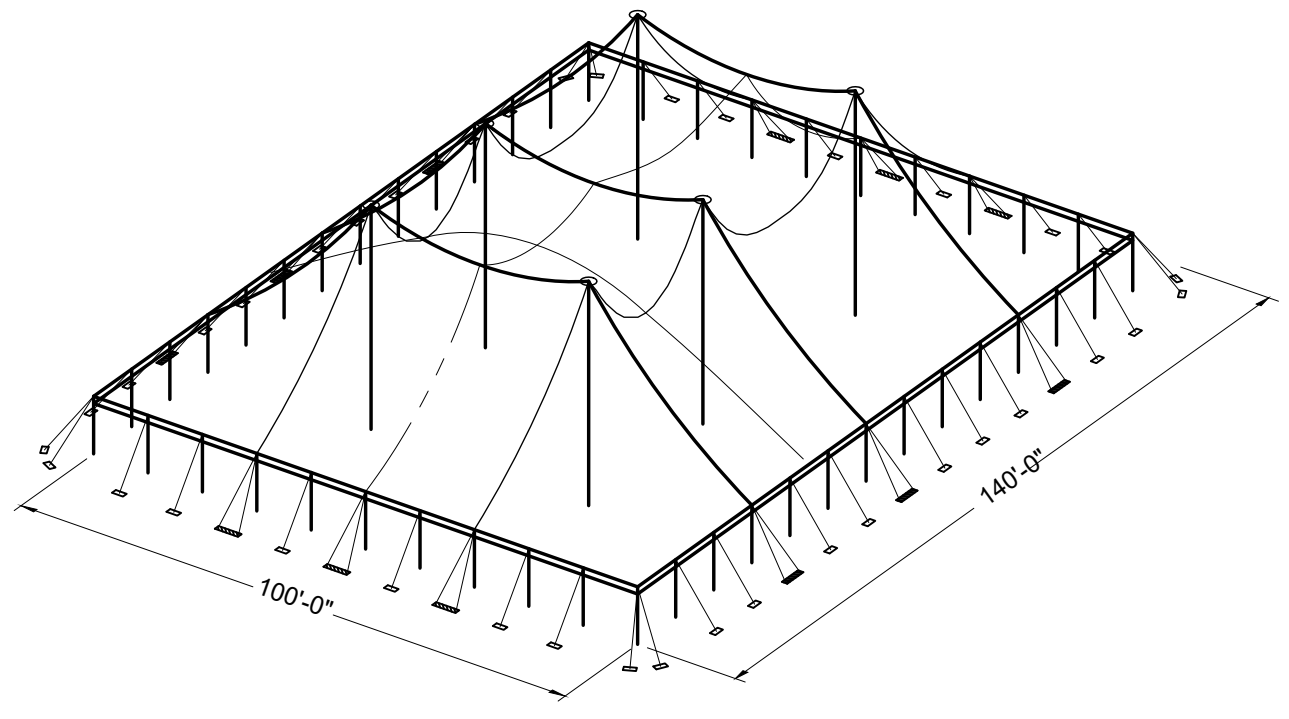
ISOMETRIC
