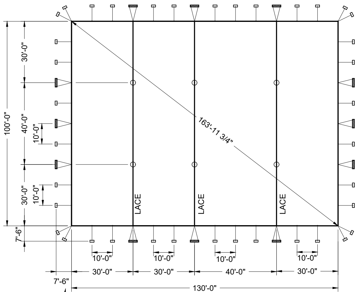
PLAN 13,000 SQ. FT.
