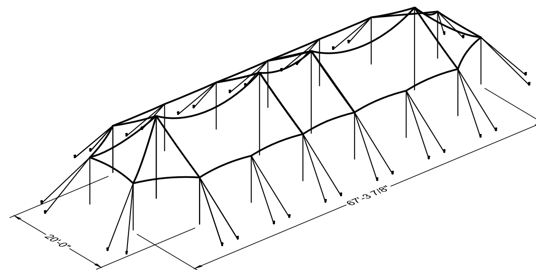
3D VIEW
