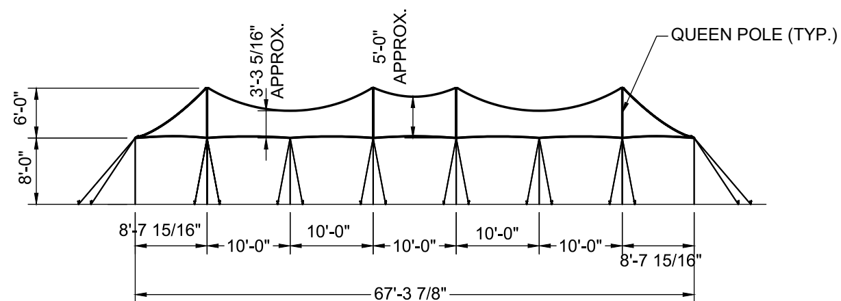
SIDE VIEW
