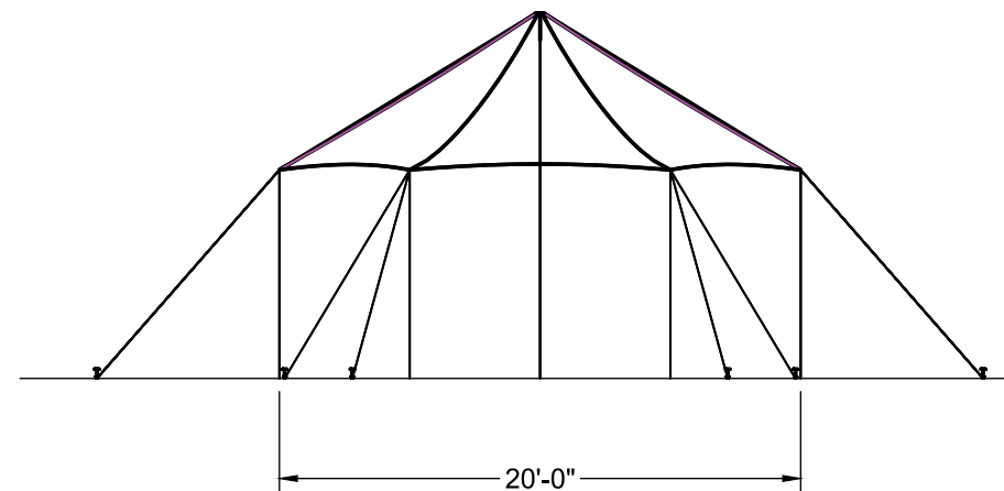
END VIEW
