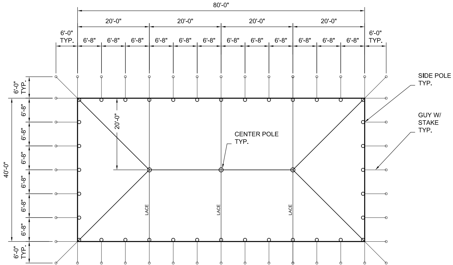
PLAN VIEW
