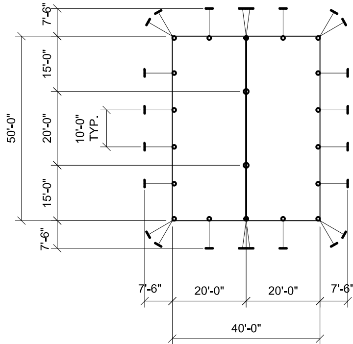
PLAN (2) ENDS
