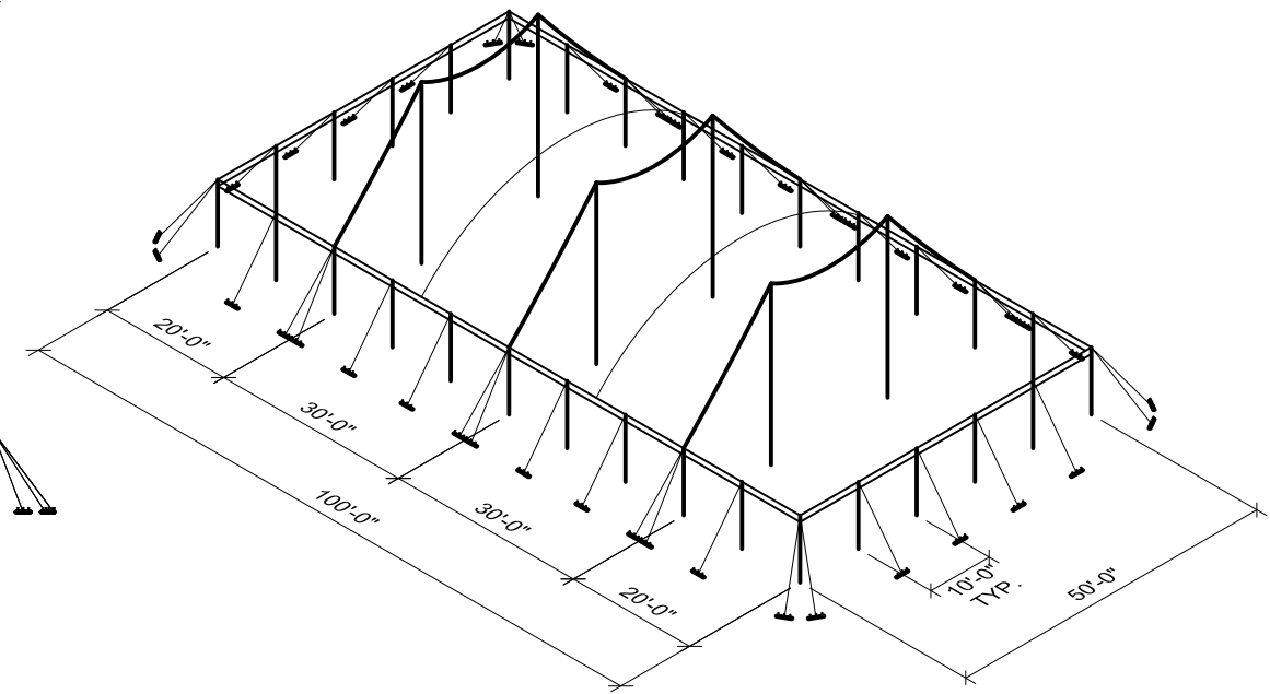
ISOMETRIC
