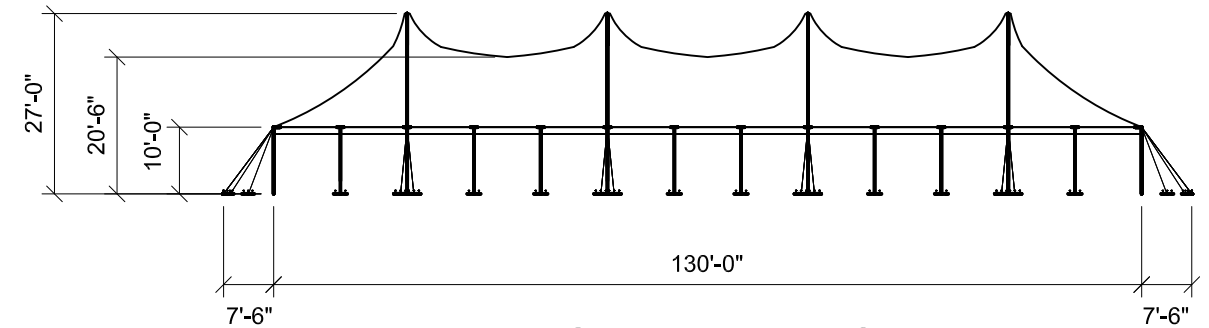
SIDE ELEVATION
