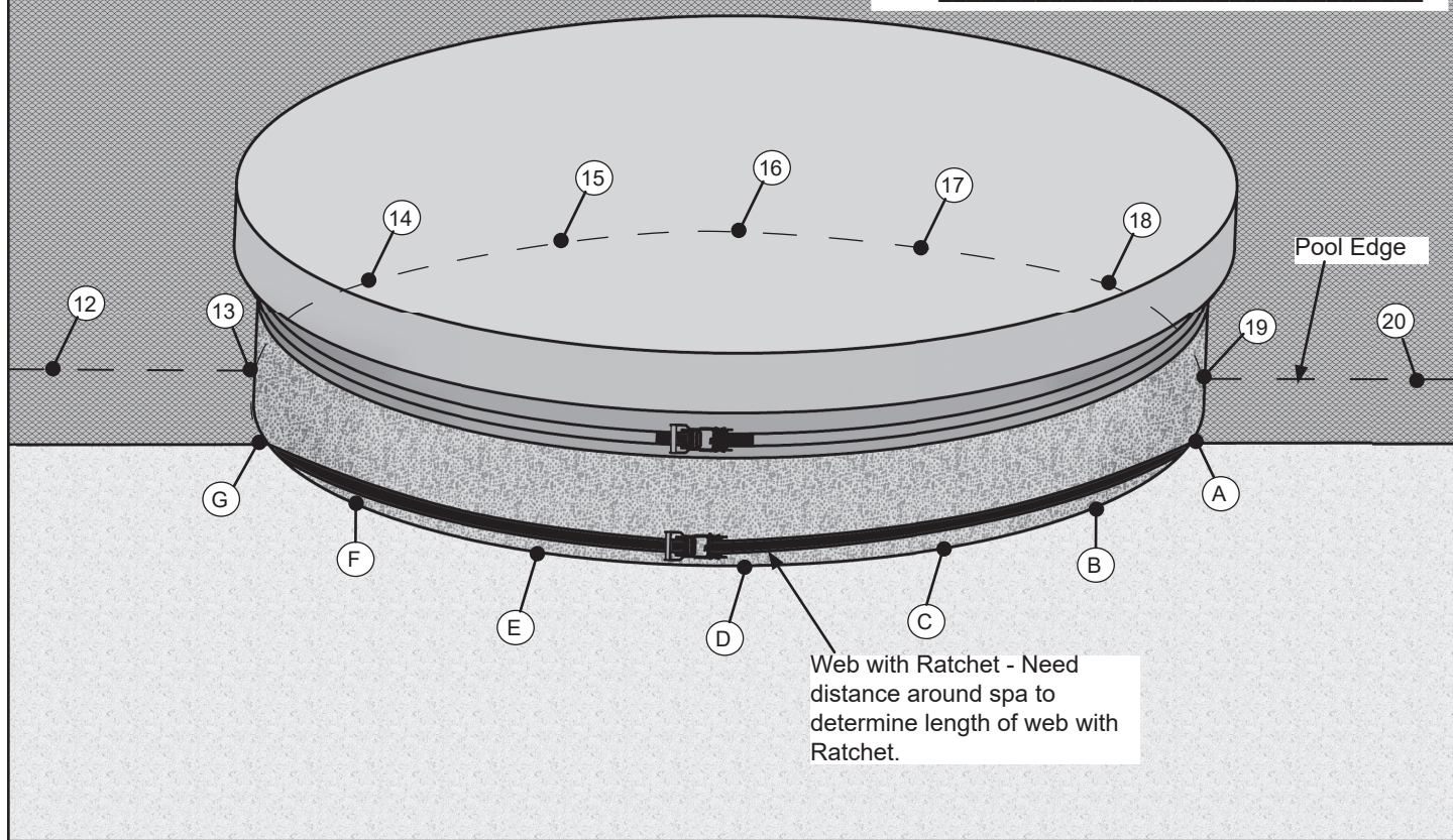
Figure B-3 SPA WITH WEB IN POCKET
