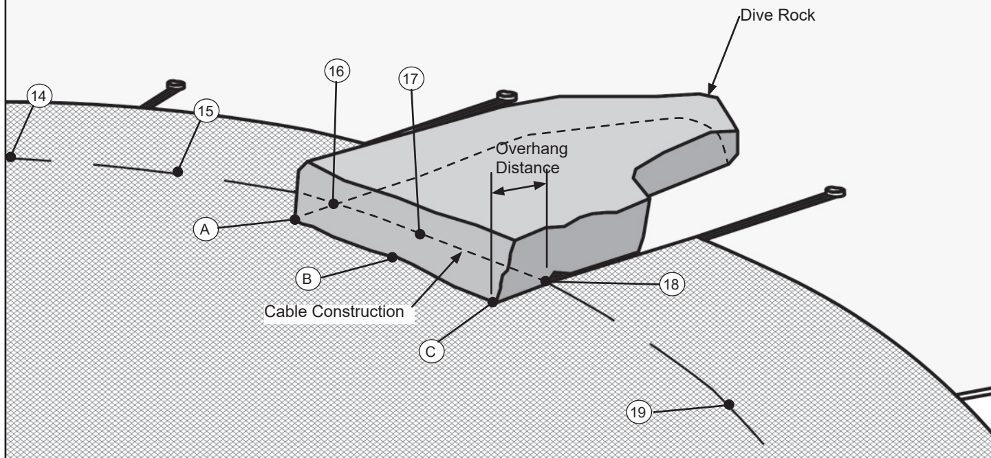
Figure A-3 DIVE ROCK WITH WEB-IN-POCKET CONSTRUCTION
