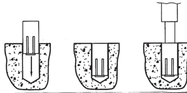
Drilling/Setting of 3/8" Drop-in Anchors
