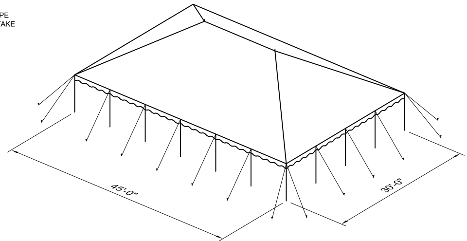
3D VIEW
