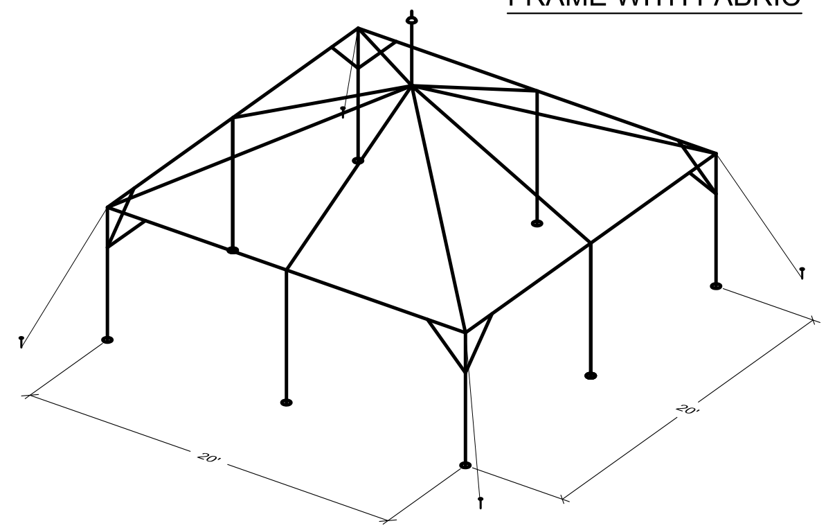
ISOMETRIC
