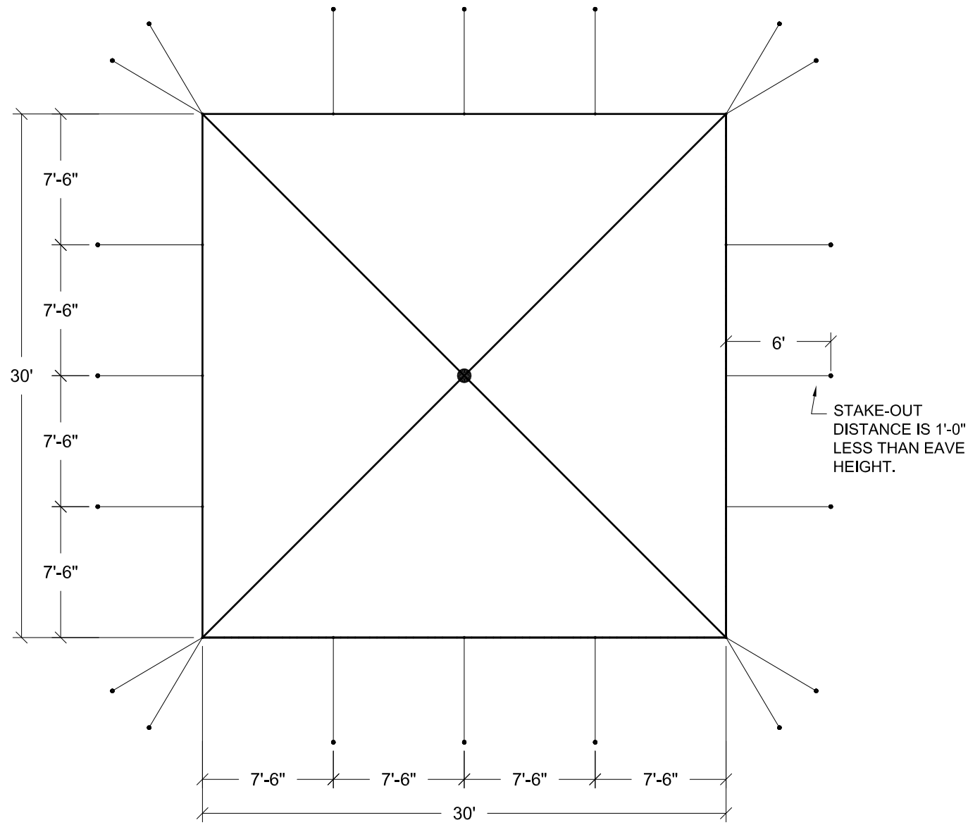
PLAN
