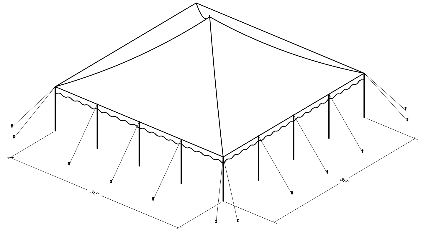
ISOMETRIC
