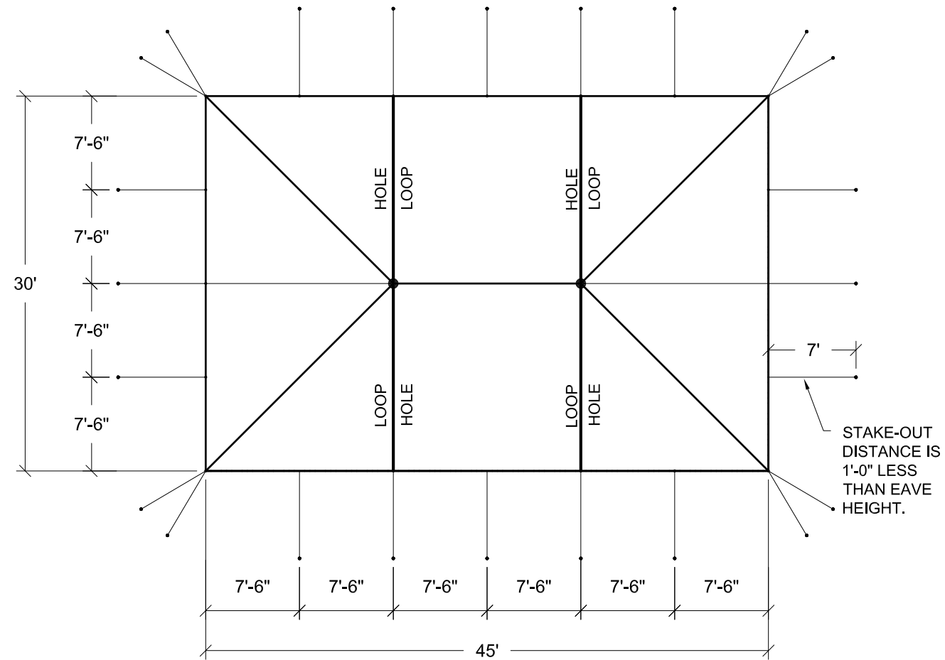
PLAN (2) ENDS & 15' MID
