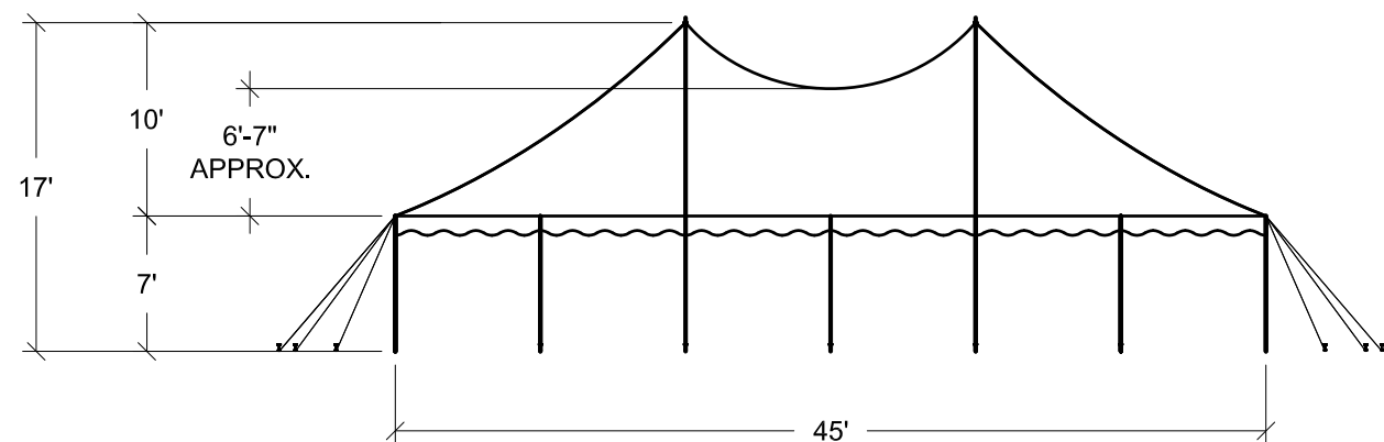
SIDE ELEVATION
