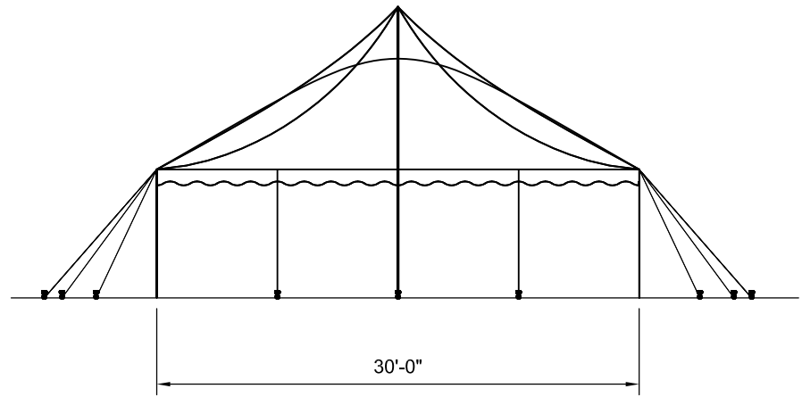
END VIEW
