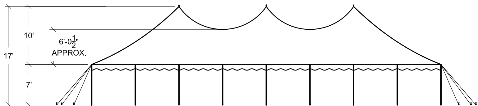
SIDE ELEVATION
