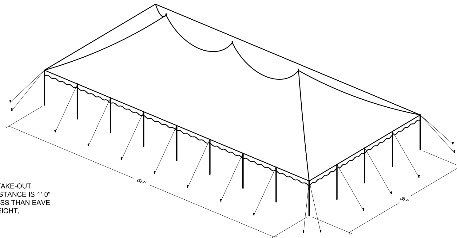
ISOMETRIC
