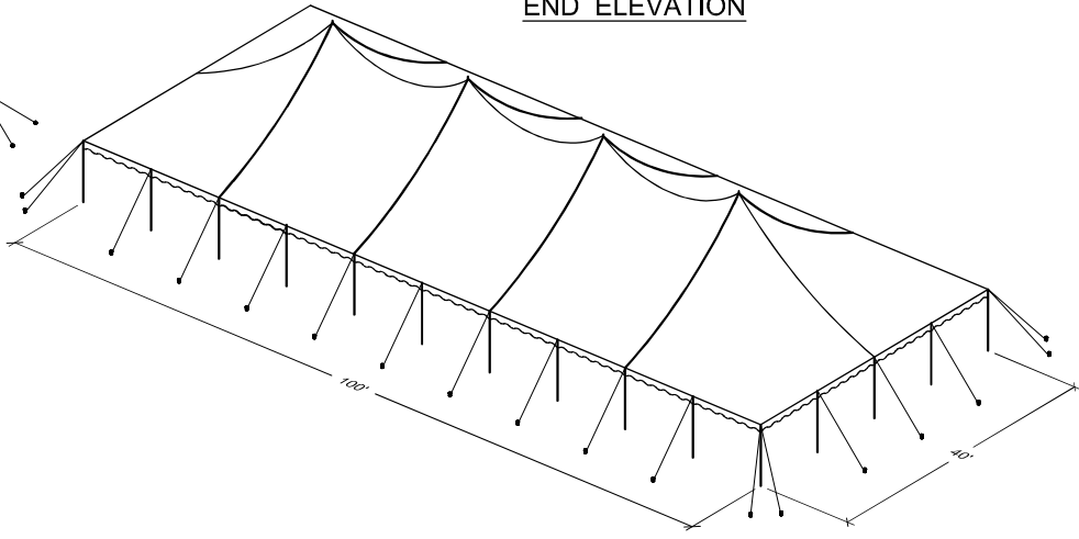
ISOMETRIC
