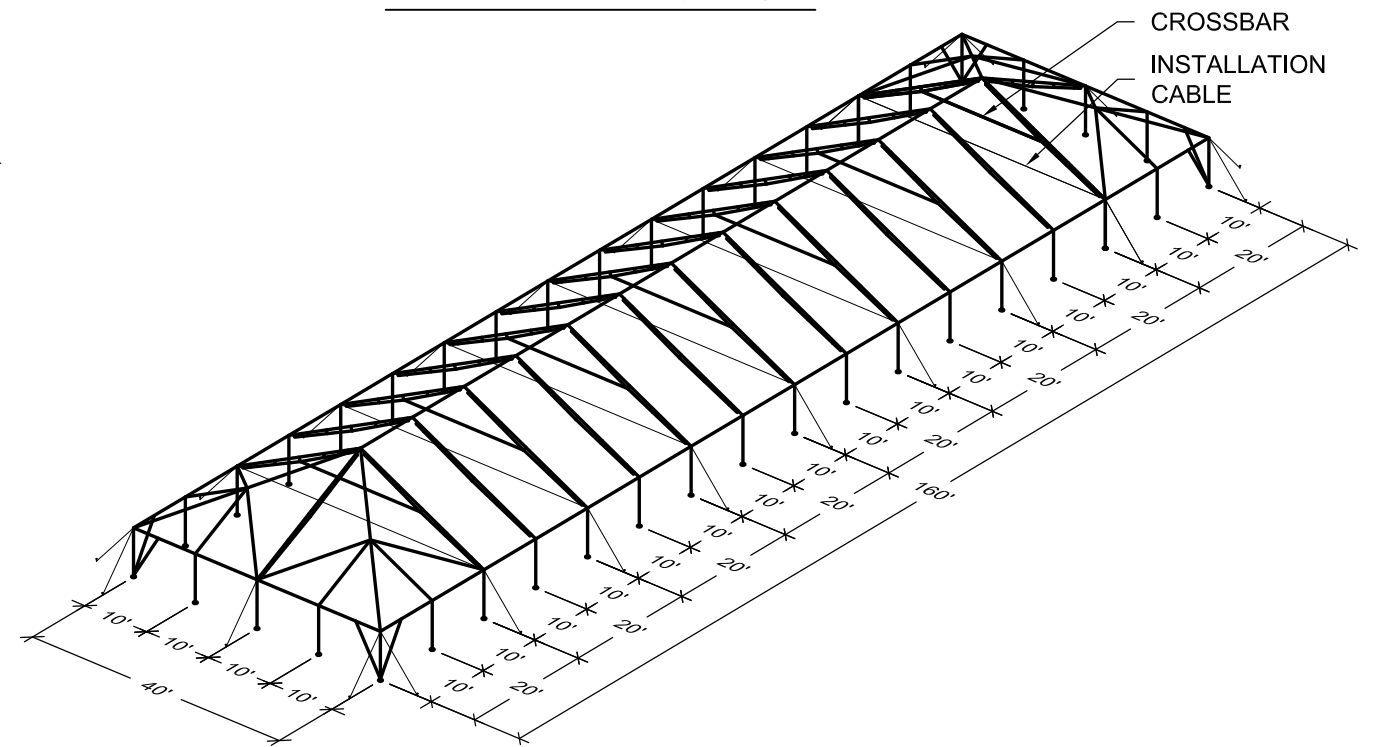
ISOMETRIC
