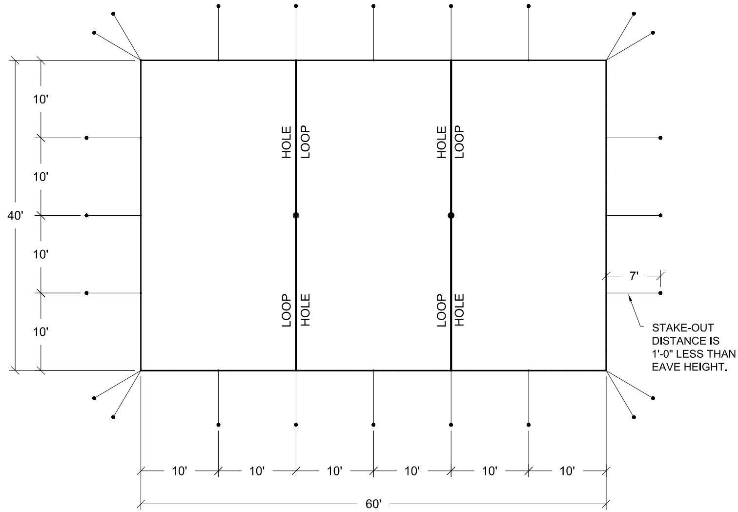
PLAN (2) ENDS & (1) 20' MID
