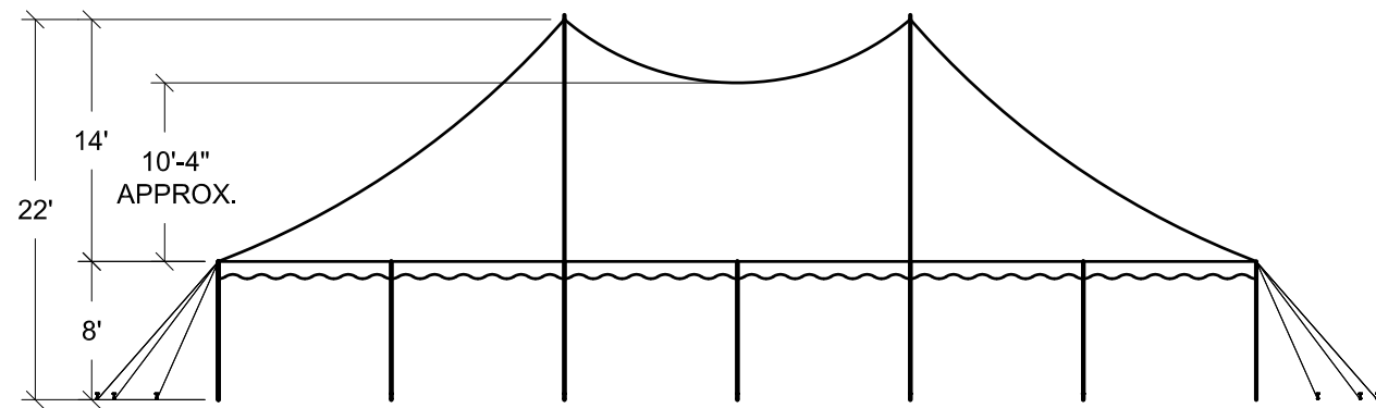
SIDE ELEVATION
