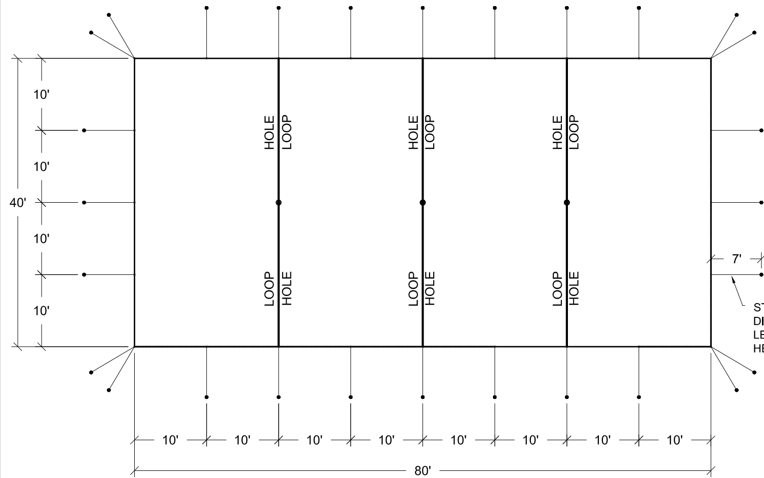
PLAN (2) ENDS & (2) 20' MIDS
