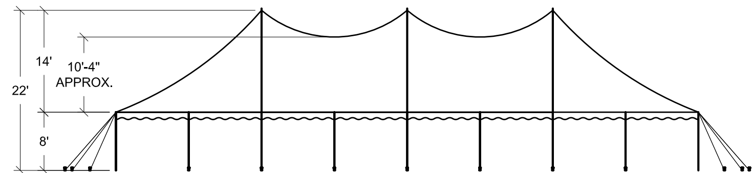
SIDE ELEVATION
