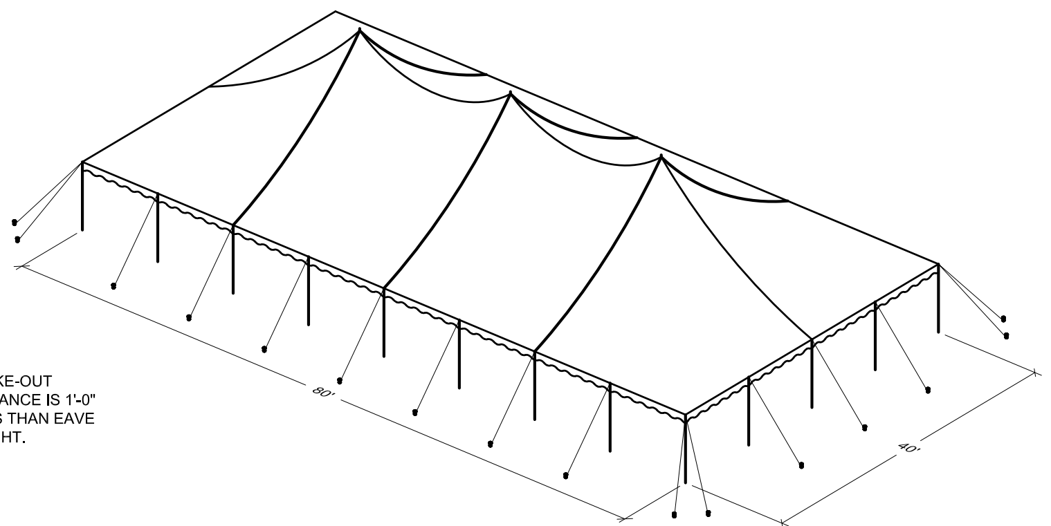
ISOMETRIC
