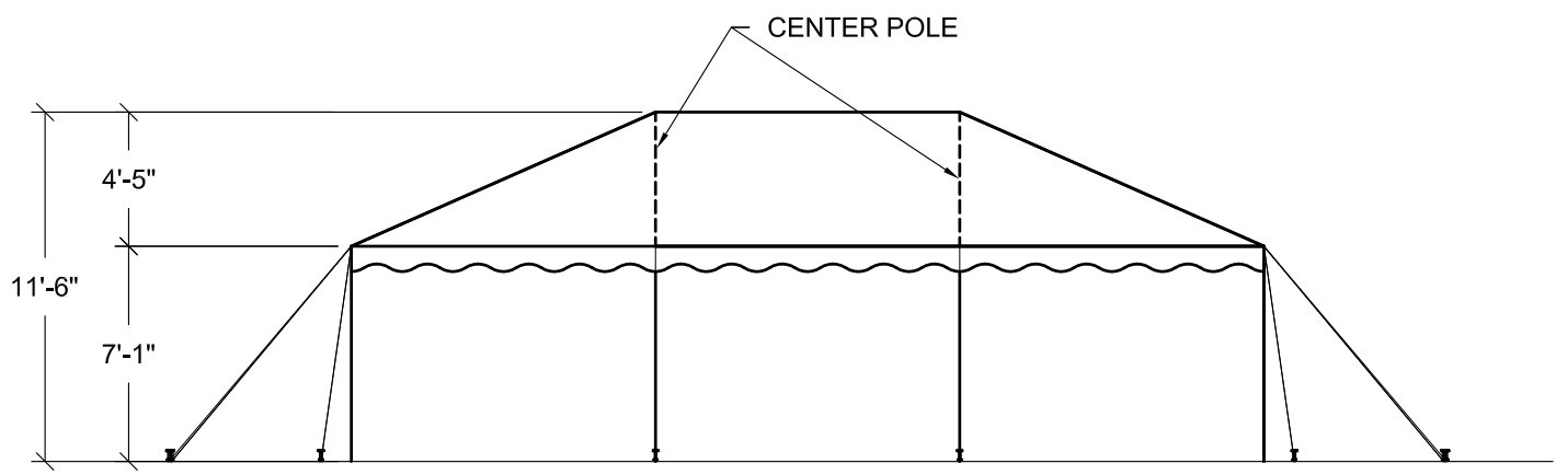
SIDE ELEVATION
