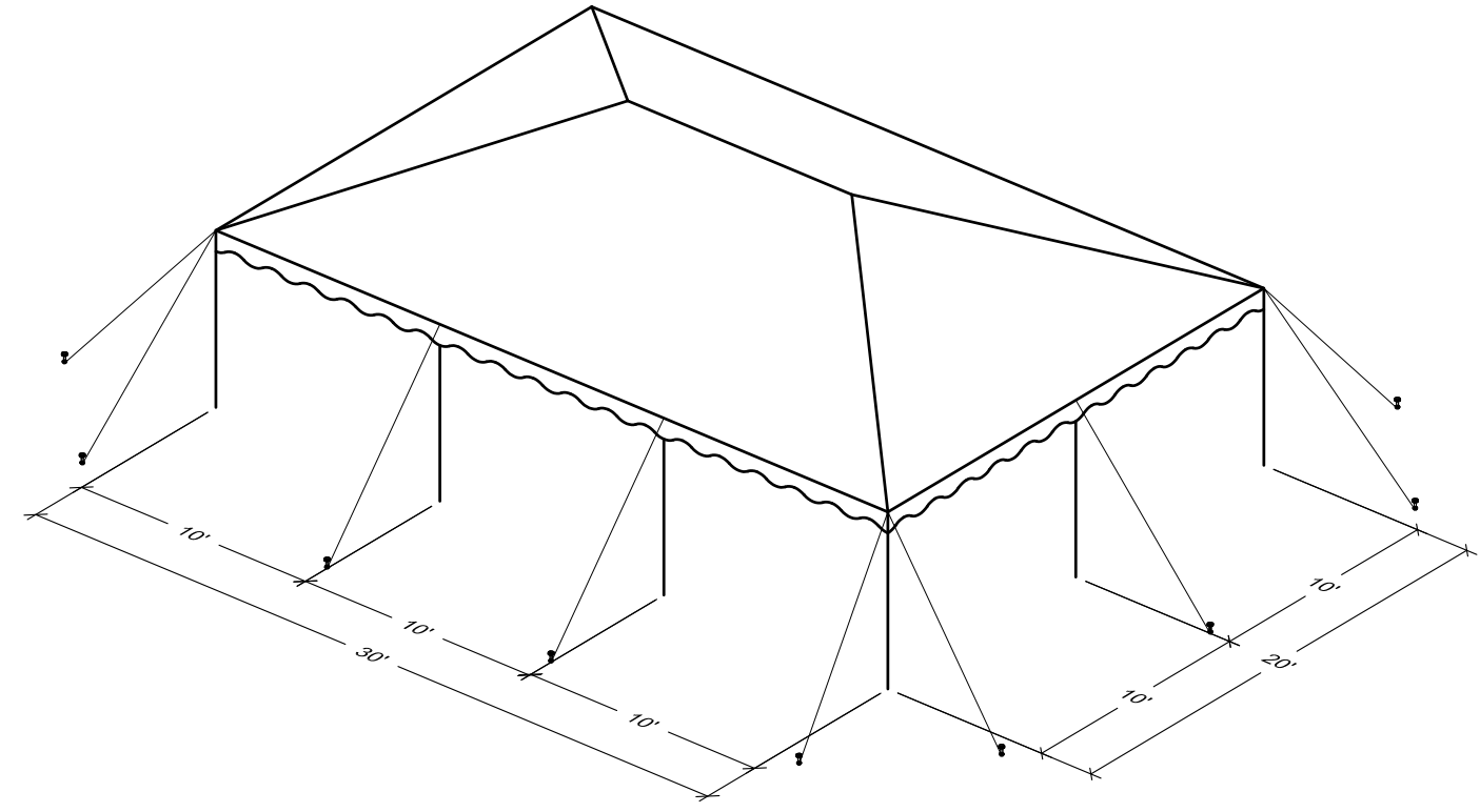
ISOMETRIC
