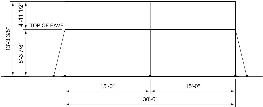
SIDE VIEW
