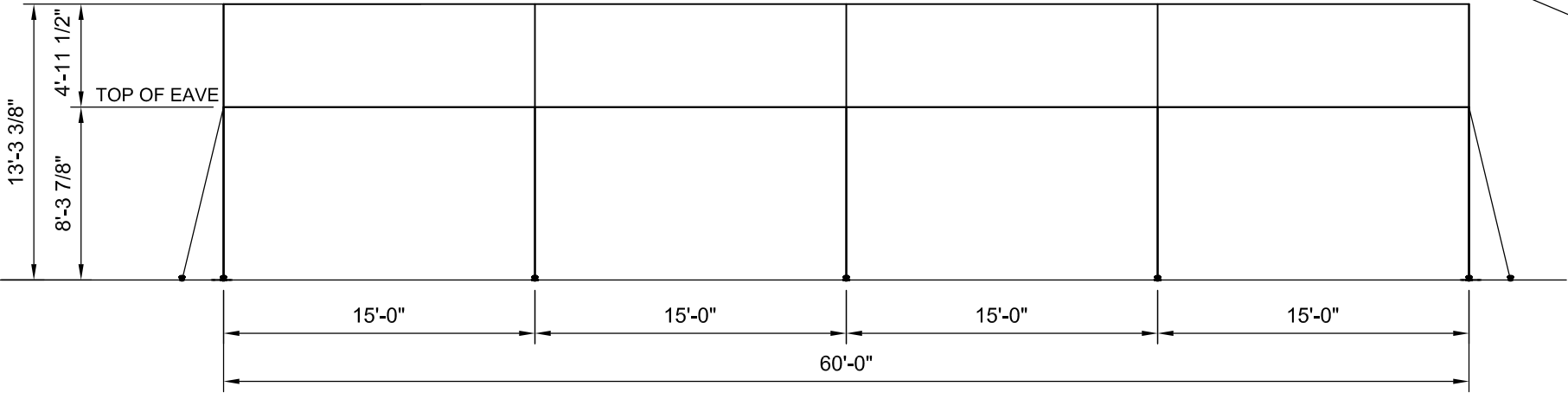
SIDE VIEW
