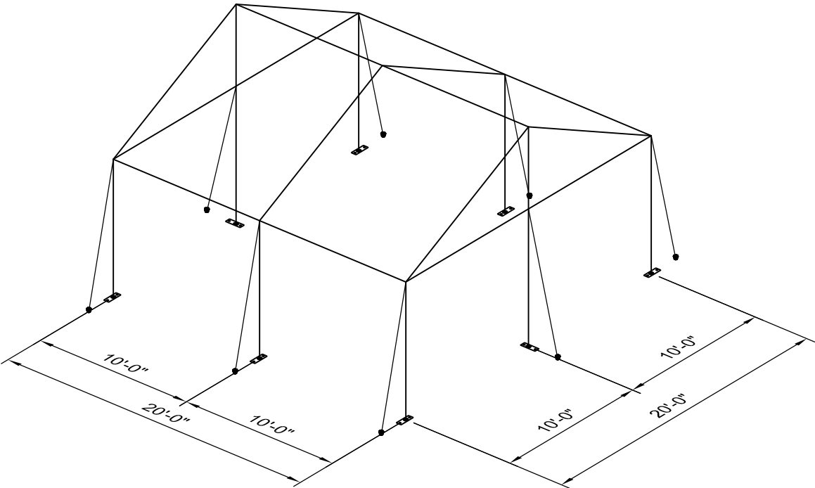
3D VIEW
