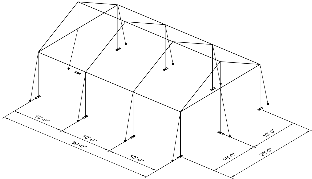
3D VIEW
