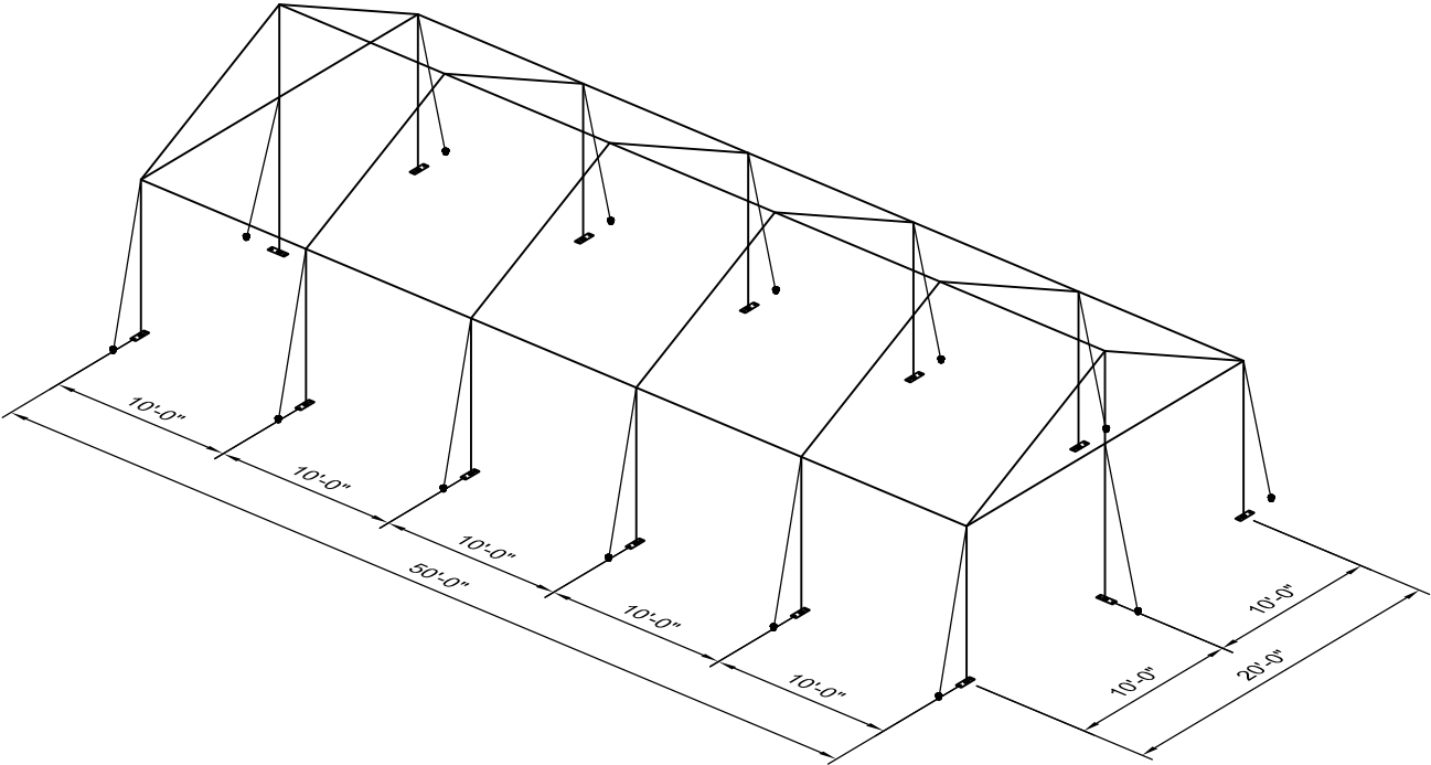
3D VIEW
