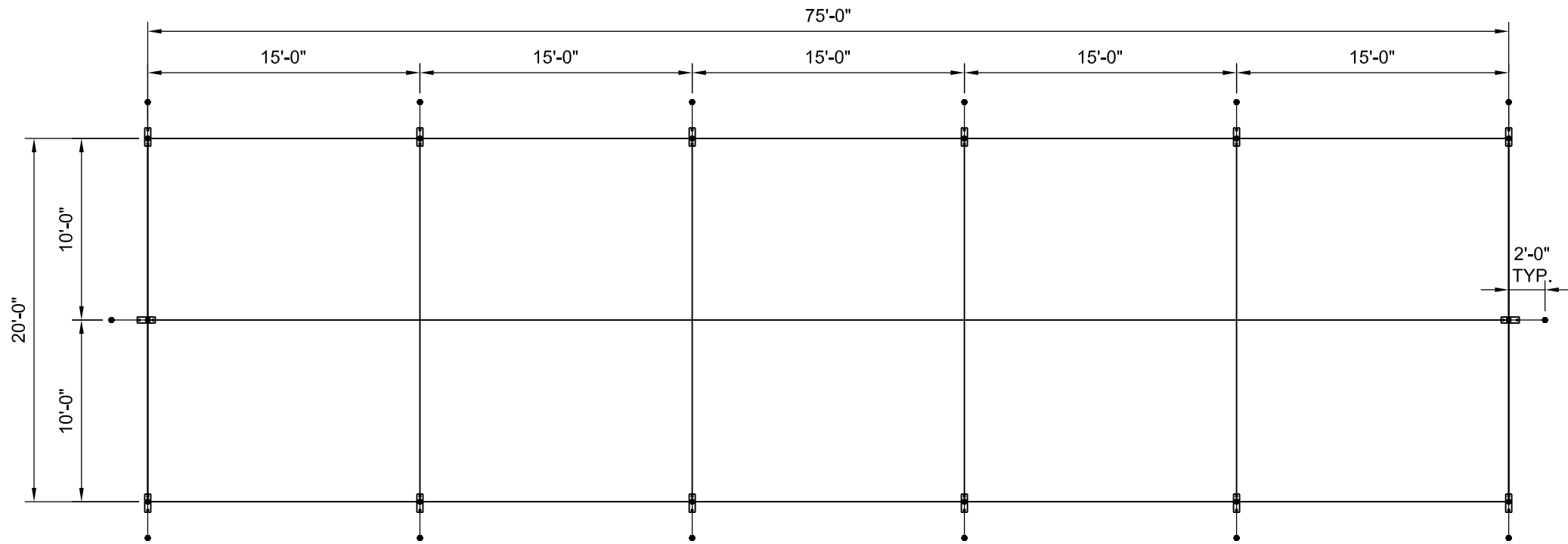
PLAN VIEW
