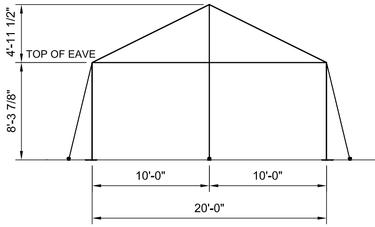
END VIEW
