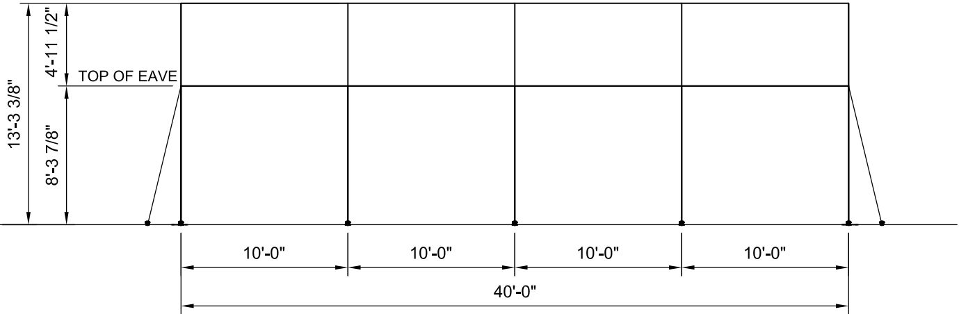
SIDE VIEW
