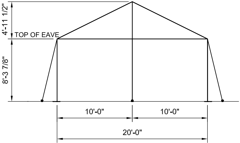
END VIEW
