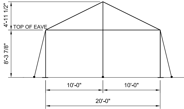
END VIEW
