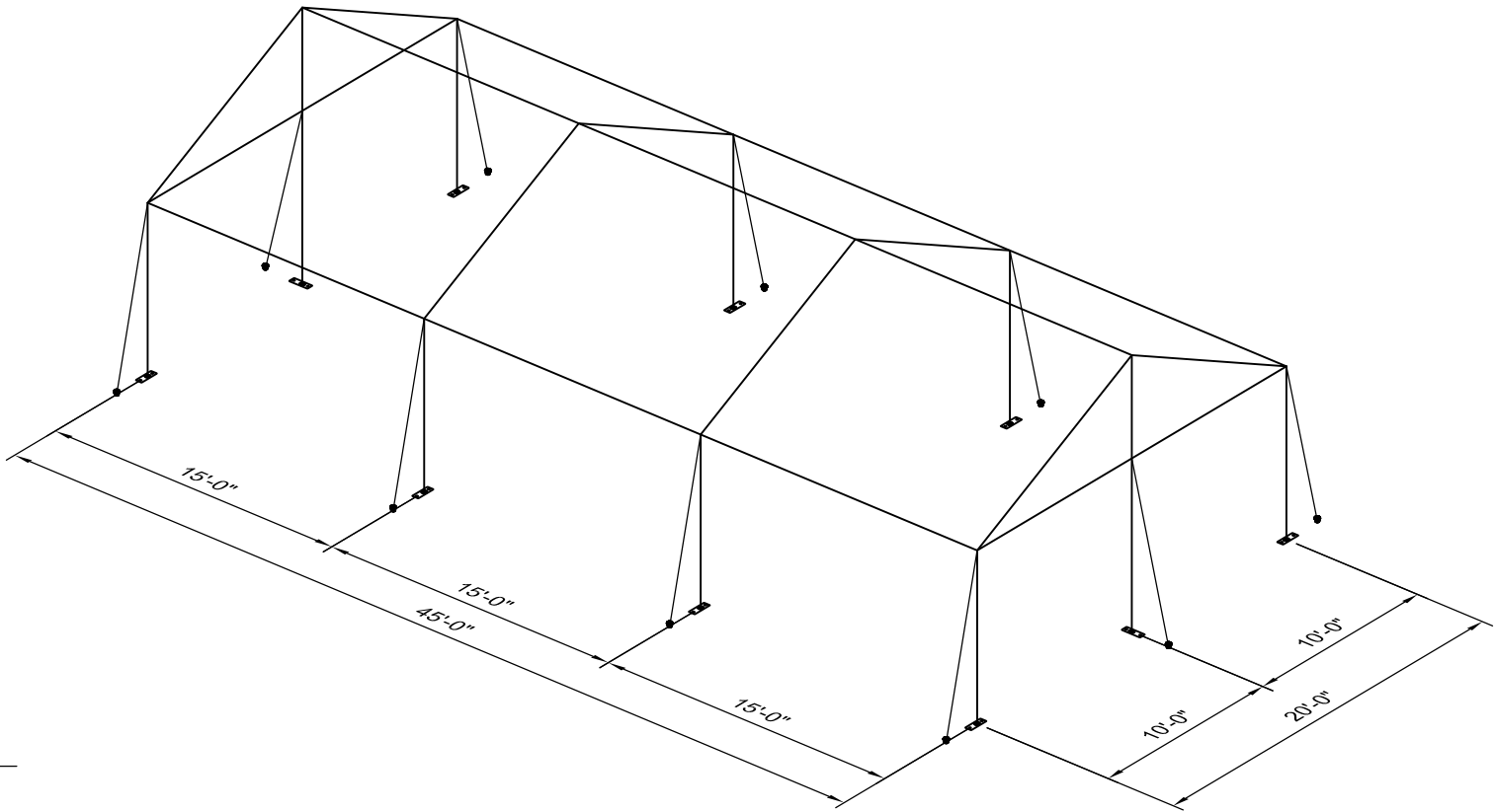
3D VIEW
