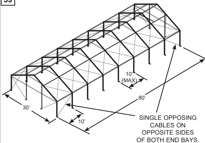
CLEARSPANS UP TO 6 OPEN BAYS
