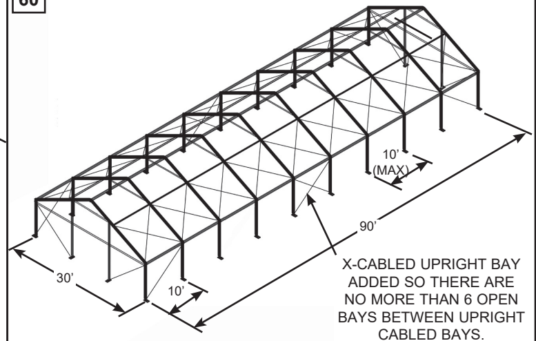
CLEARSPANS EXCEEDING 6 OPEN BAYS BETWEEN UPRIGHT CABLED BAYS.
