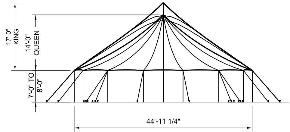
END VIEW
