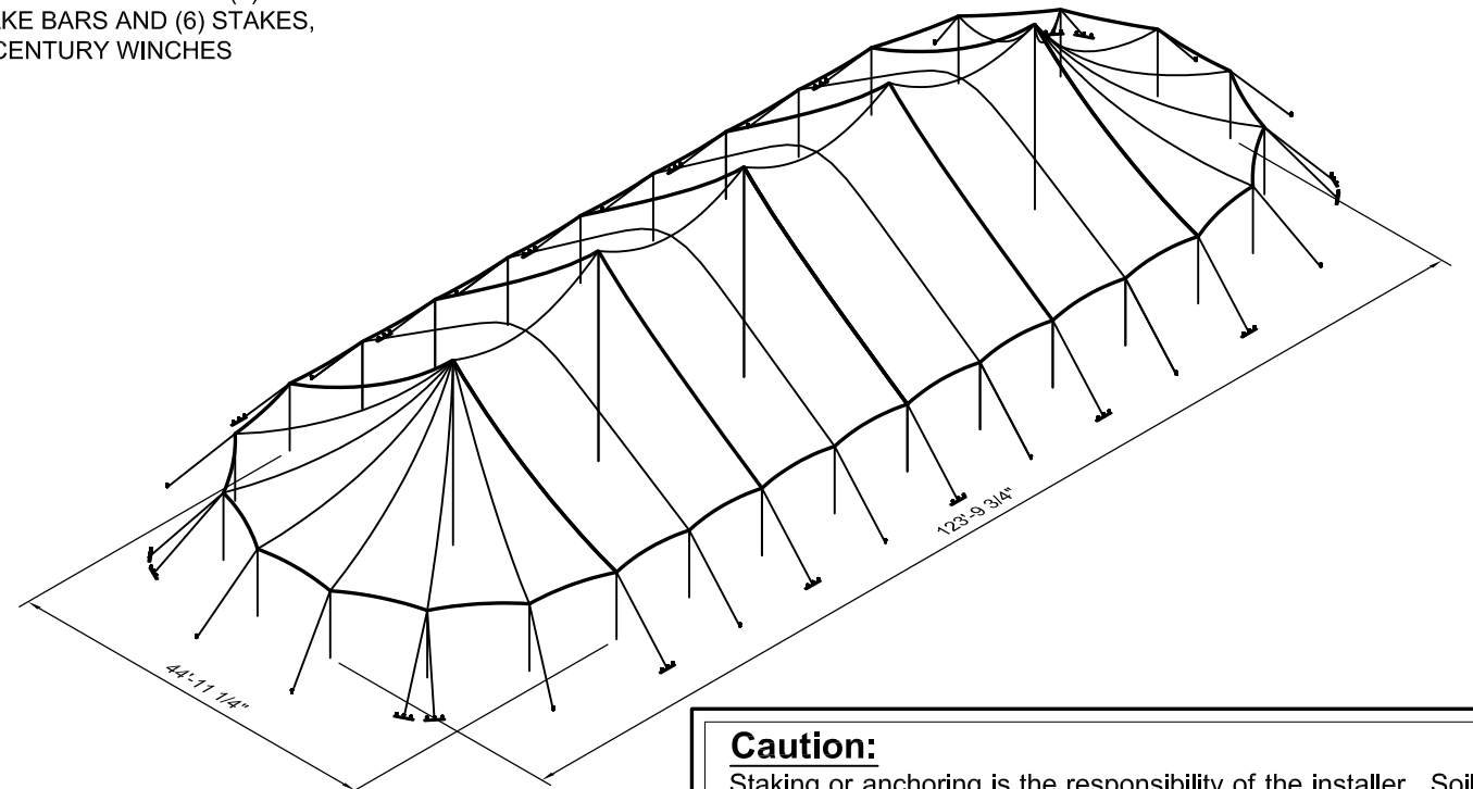
3D VIEW
