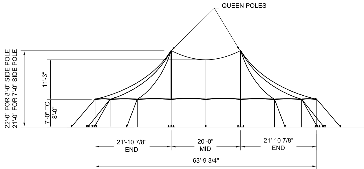
SIDE VIEW
