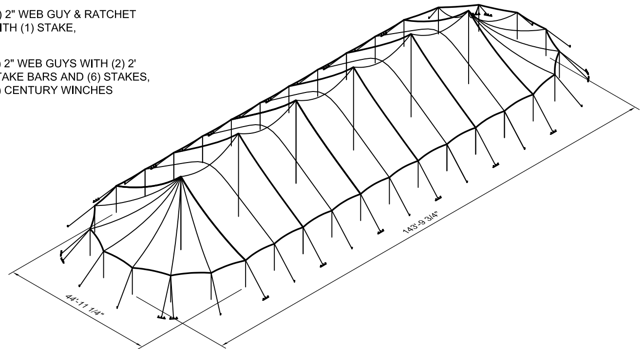
3D VIEW
