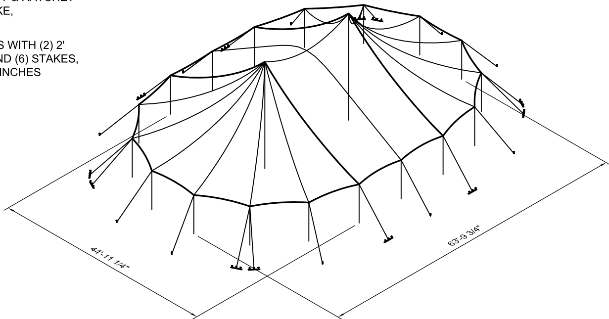
3D VIEW
