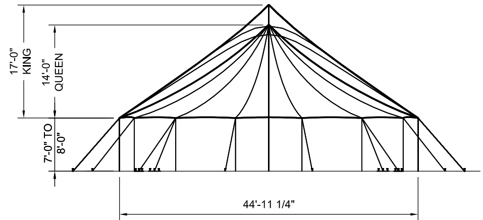
END VIEW
