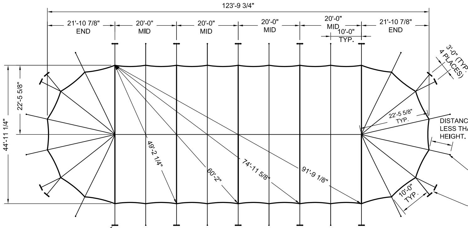
PLAN VIEW
