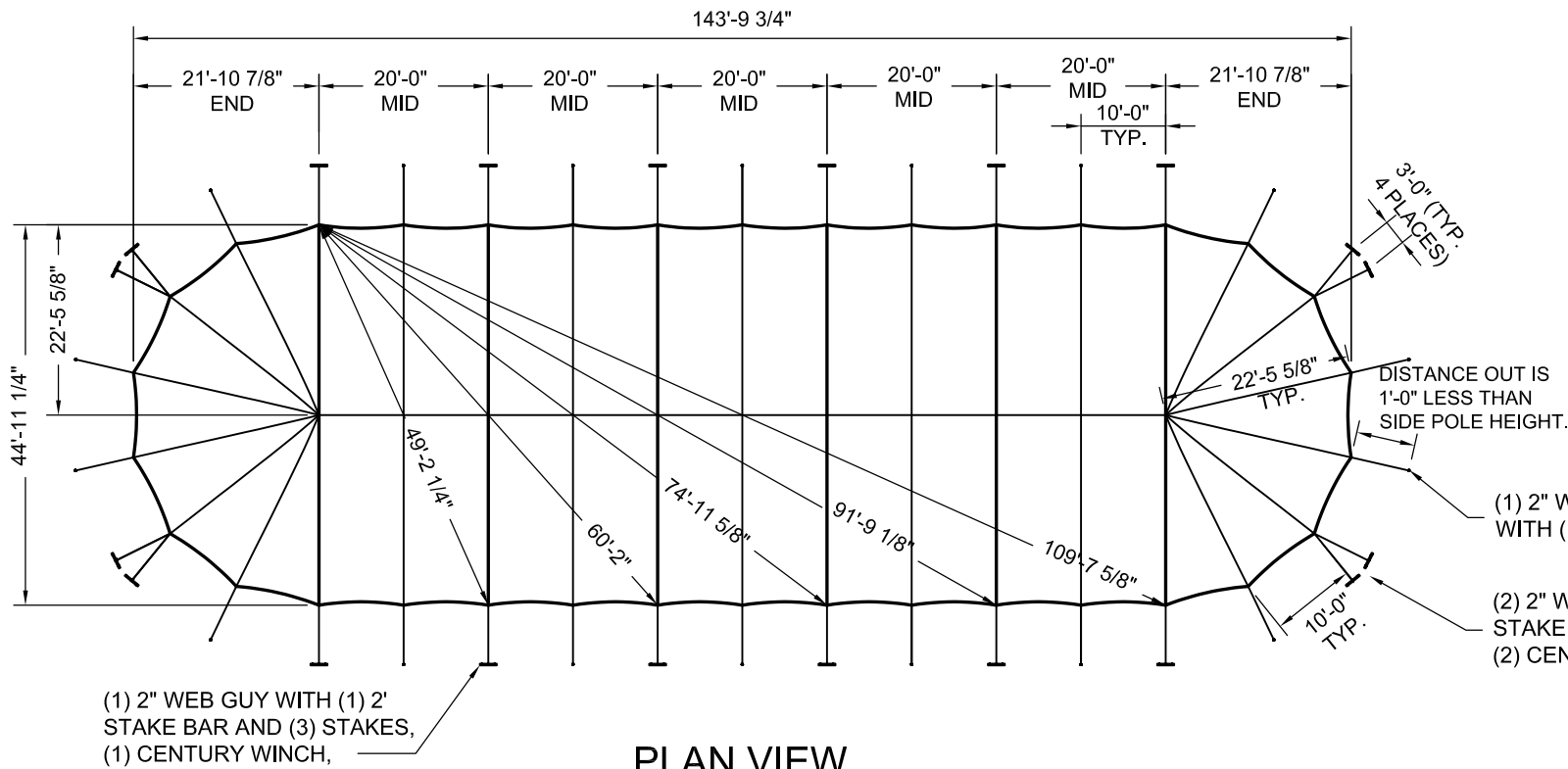
PLAN VIEW
