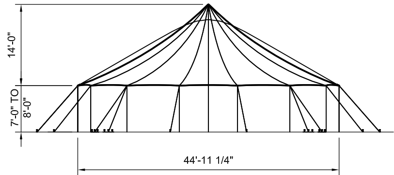
END VIEW
