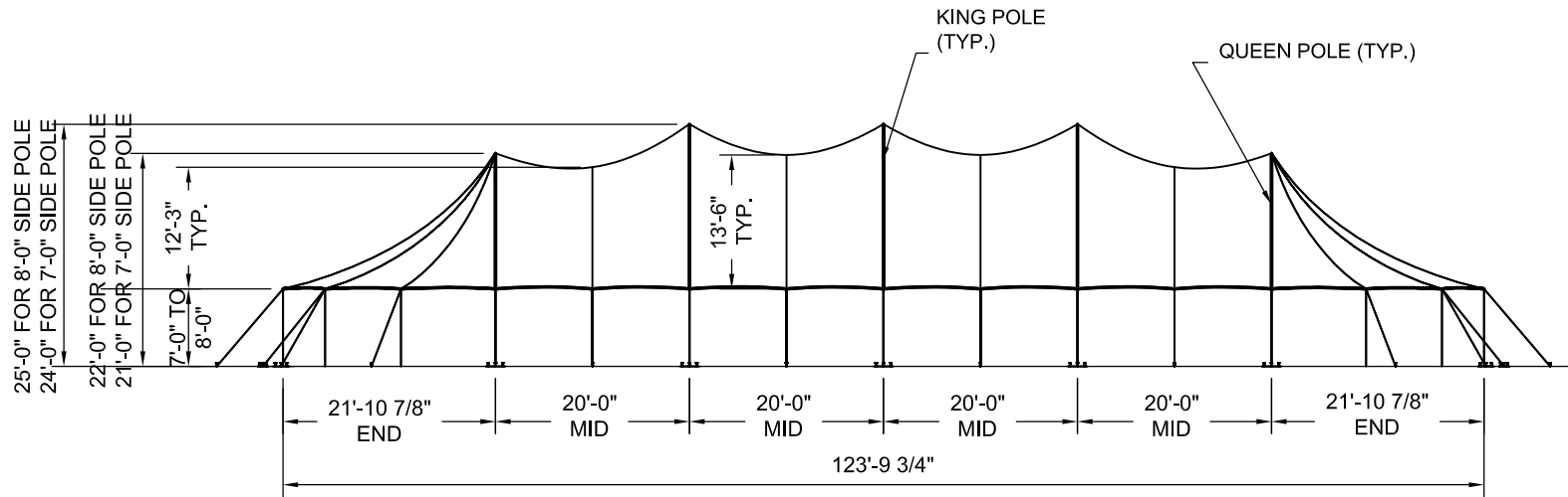
SIDE VIEW
