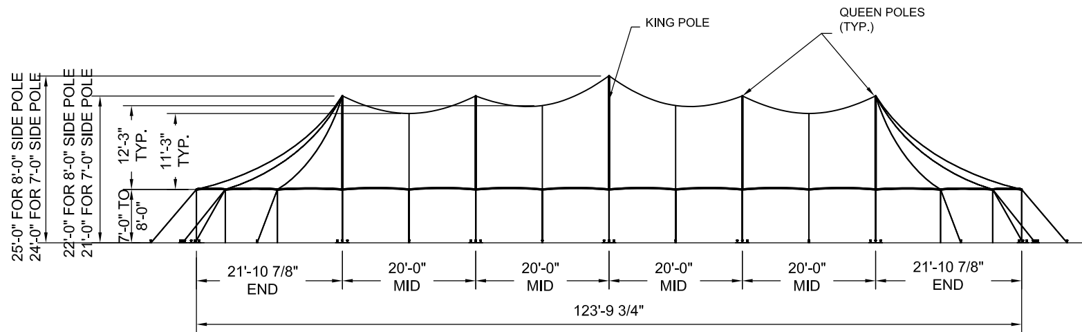
SIDE VIEW
