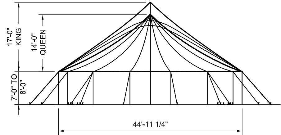
END VIEW
