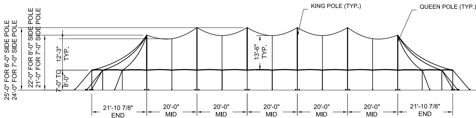
SIDE VIEW
